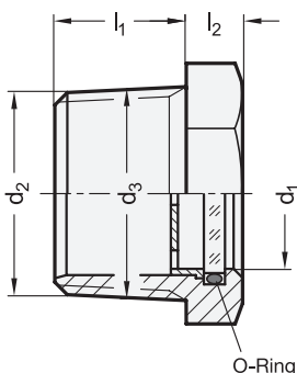
O-Ring
